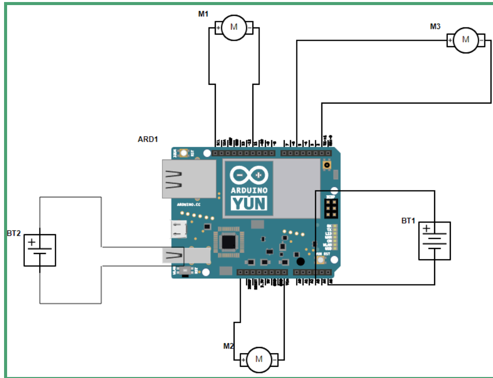
Figure 9: Schematic Diagram
