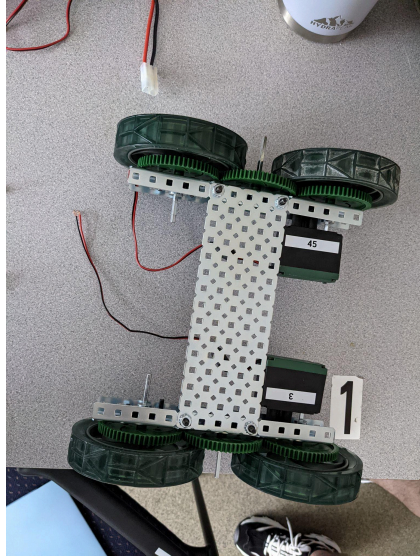
Figure 5: Chassis of DemeterBot
