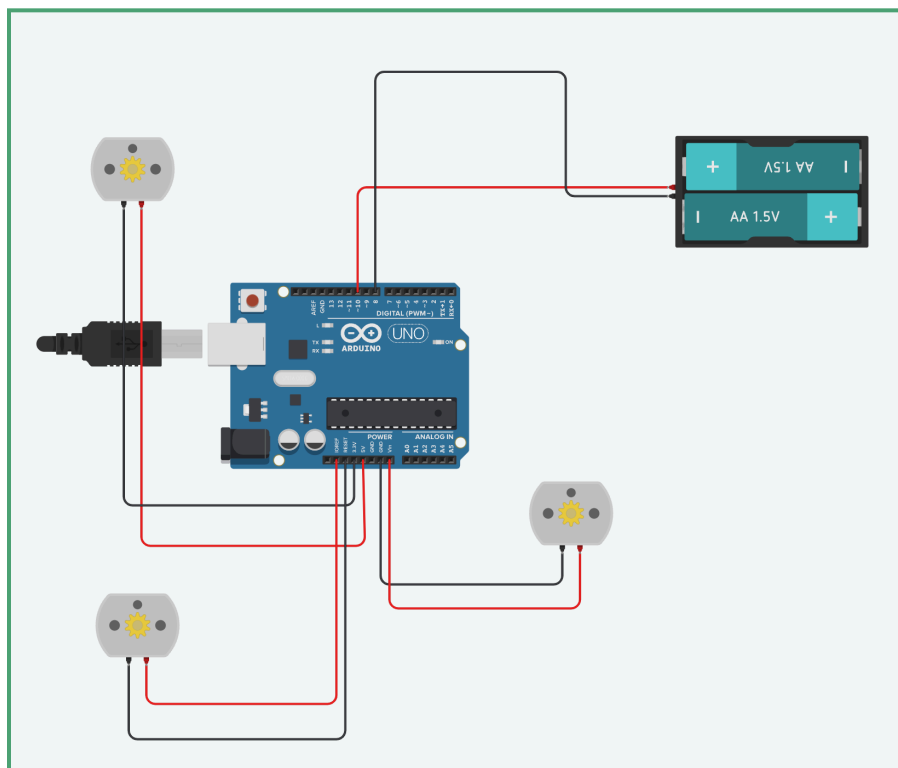
Figure 8: Circuit Diagram
