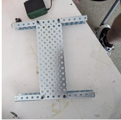
Figure 4: Skeletal Chassis
